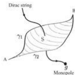
Figure 8. A Dirac string is enclosed between two generic paths \gamma_1 and \gamma_2 starting at A, ending at B, and forming the boundary of the surface S.
