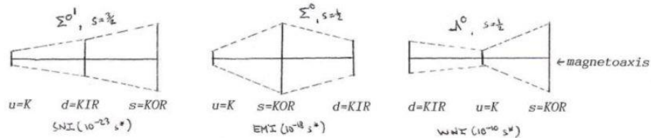
The importance of the uds -lambda quantum geometry
