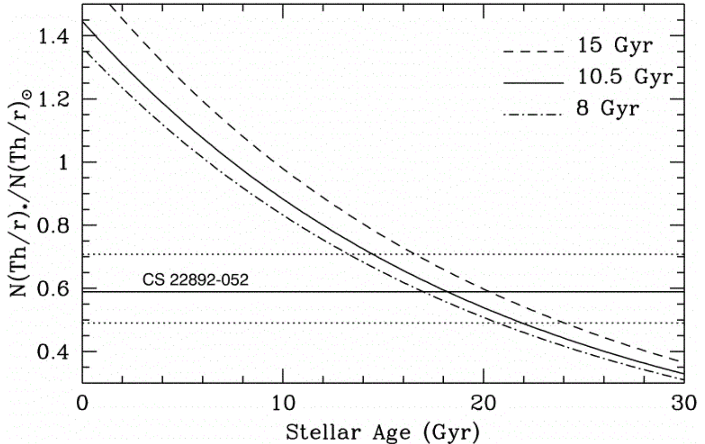
FIG. 8. —Age dependence of the observed Th/r ratio (in units of the observed solar system value), based on a simple model of chemical evolution and three different assumed ages for the Galactic disk. Galactic disk ages of 8, 10.5, and 15 Gyr are indicated. The horizontal lines represent the observed Th/r ratio in CS 22892-052 with 1\sigma uncertainty; the best-fit age is 18 Gyr, with an acceptable range from 14 to 22 Gyr.
